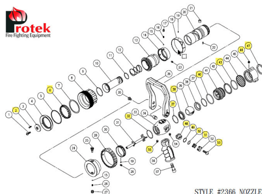
SERVICE PART LIST FOR #2366 NOZZLE
